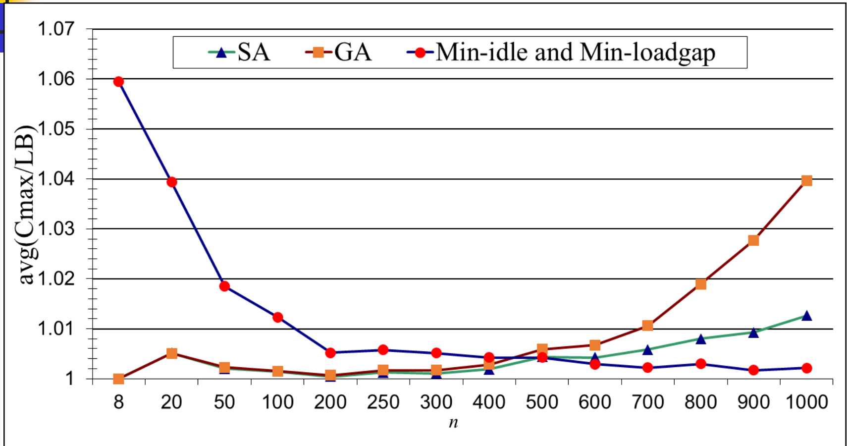
Comparison of the average values of the relation C_{max}/LB of Algorithms Min-idle and Min-loadgap with Algorithms SA and GA.
